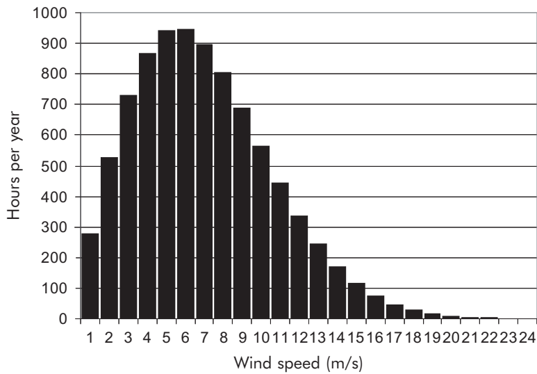
Figure 4 – Wind speed distribution, average wind speed 7 m/s and Weibull shape factor of 2
