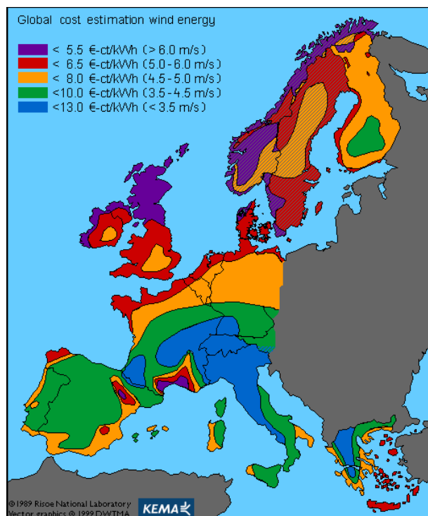
Figure 1 – Overview of European Wind Atlas (No data is available for the Balkans and Eastern Europe)
