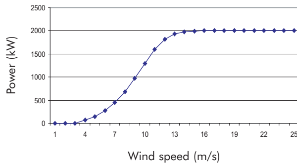
Figure 3 – Power/wind speed curve of a 2 MW wind turbine (without noise reduction measures)
