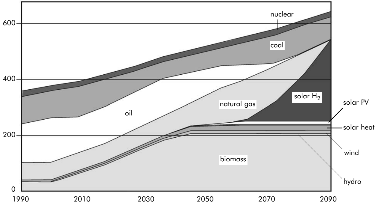
Figure 7 - Energy resources mix required if atmospheric CO 2 concentrations are to be stabilised at 400 ppm
