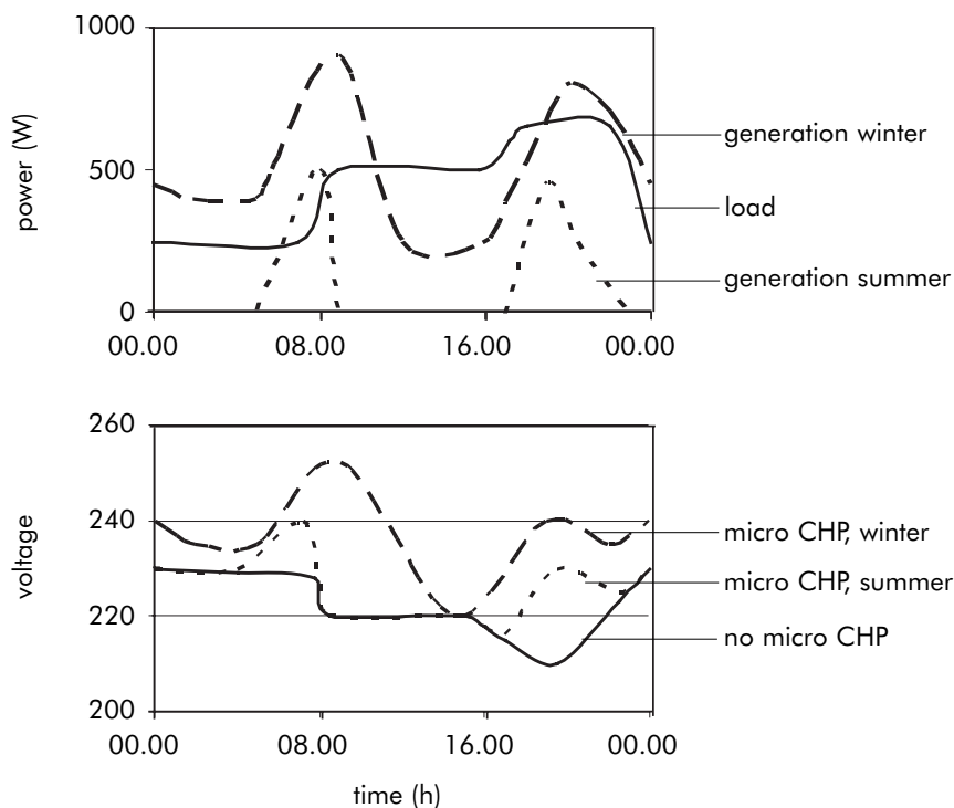
Figure 13 – Power variations and voltage fluctuations due to micro CHP installation
