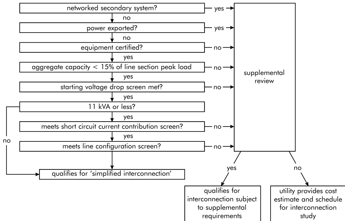
Figure 4 - An example flowchart of requirements for interconnecting DG resources
