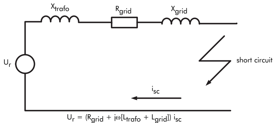
Figure 11 – Equivalent circuit of a grid branch with a short circuit
