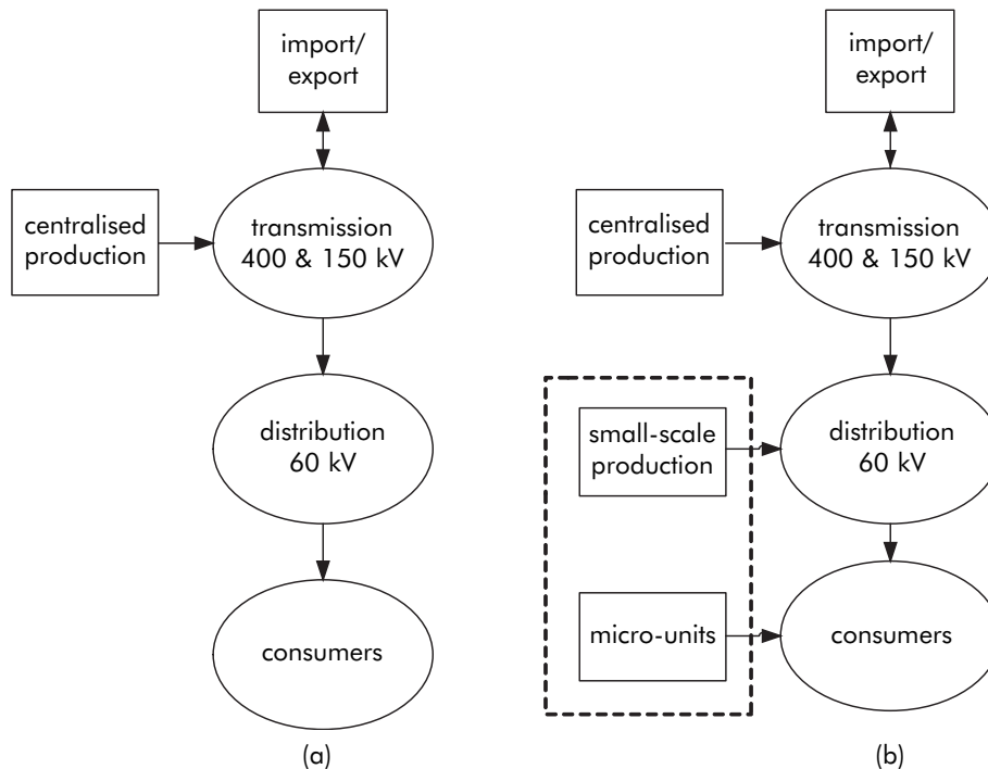
Figure 5 – a) A uni-directional centrally delivered power generation system and b) a bi-directional system with distributed generation
