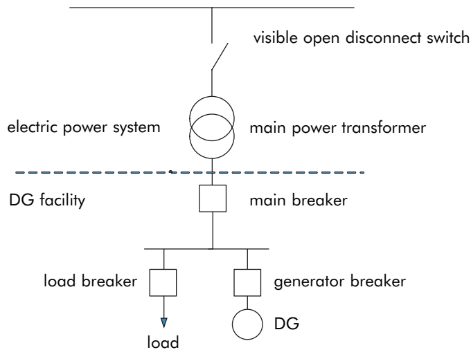
Figure 3 - Interconnection of DG technologies based on synchronous or asynchronous generators
