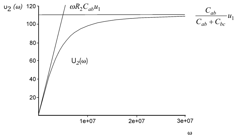
Figure 13 - Frequency behaviour of the capacitive coupling
