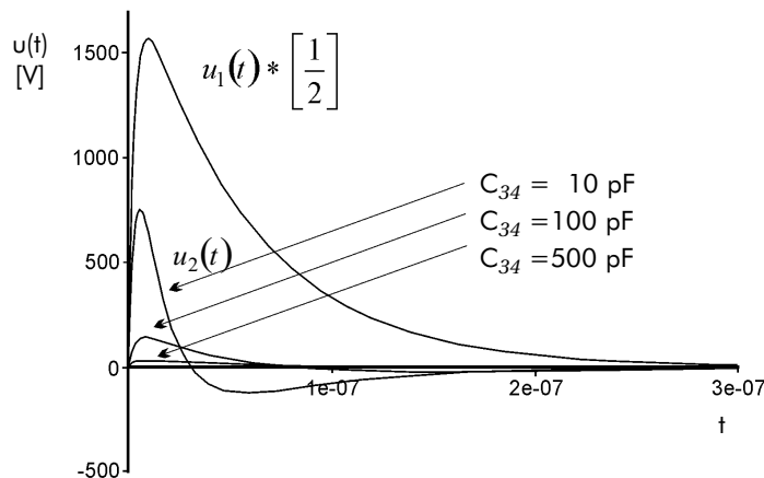
Figure 16 - Shielding of a burst pulse by shields of a different internal capacitive coupling
