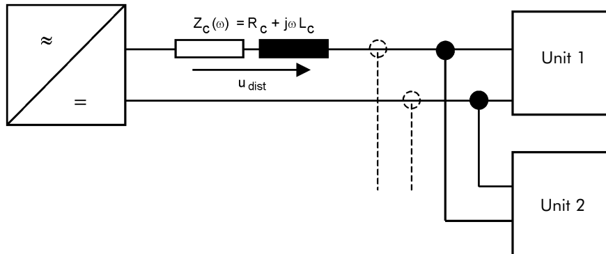
Figure 3 - Impedance coupling, simple model
