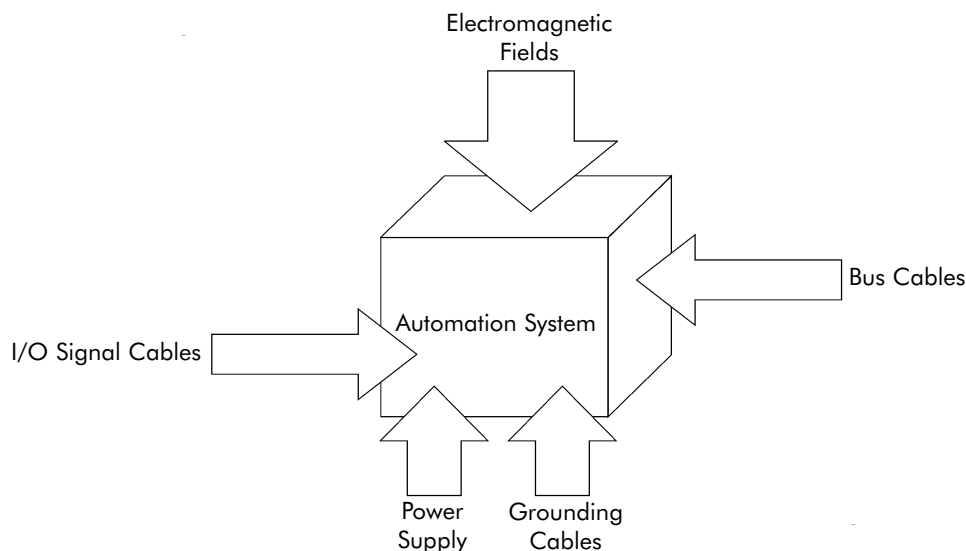
Figure 18 - Various couplings paths of an automation system
