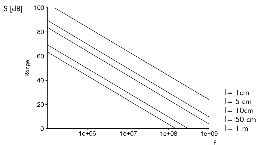
Figure 17 - Shielding effectiveness of a slot of various lengths as a function of frequency
