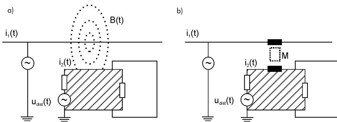
Figure 4 - Inductive coupling a) field model, b) equivalent circuit
