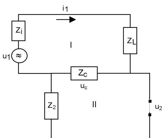
Figure 2 - Impedance coupling
