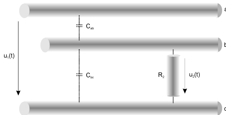
Figure 12 - Three line model for capacitive coupling
