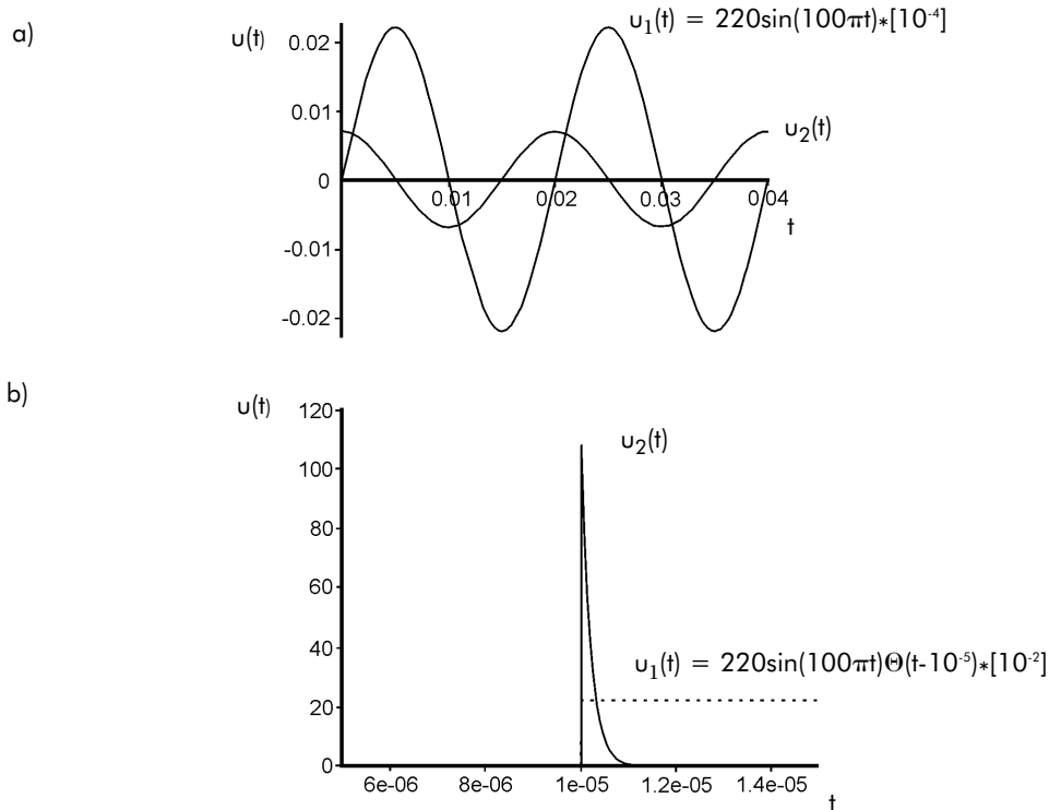
Figure 14 - Capacitive coupled signals of a) a 50 Hz sine wave, b) a phase-angle control dimmer
