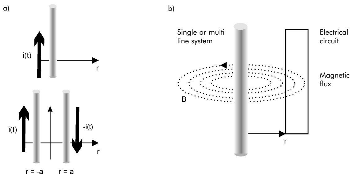
Figure 5 - a) A single and a go-and-return line as sources of a magnetic field b) an electrical circuit as a drain
