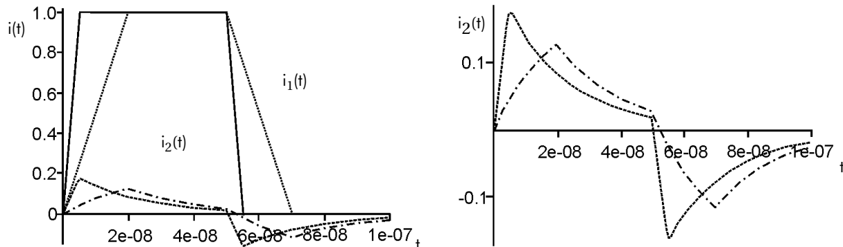
Figure 9 - Inductive coupling of slow and fast trapezoidal currents
