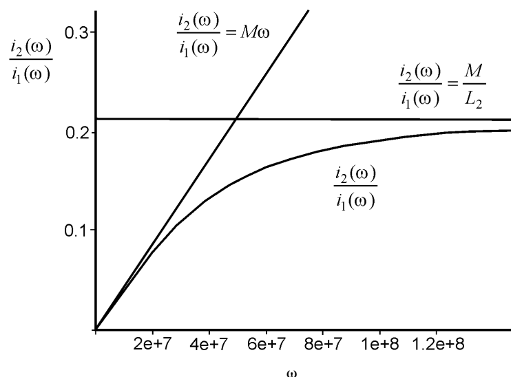
Figure 8 - Case study of the transfer function of the current
