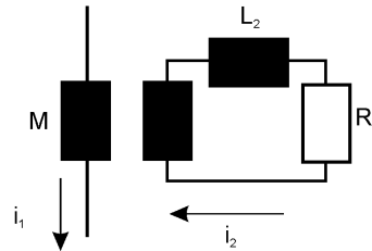
Figure 7 - Equivalent circuit for the inductive coupling
