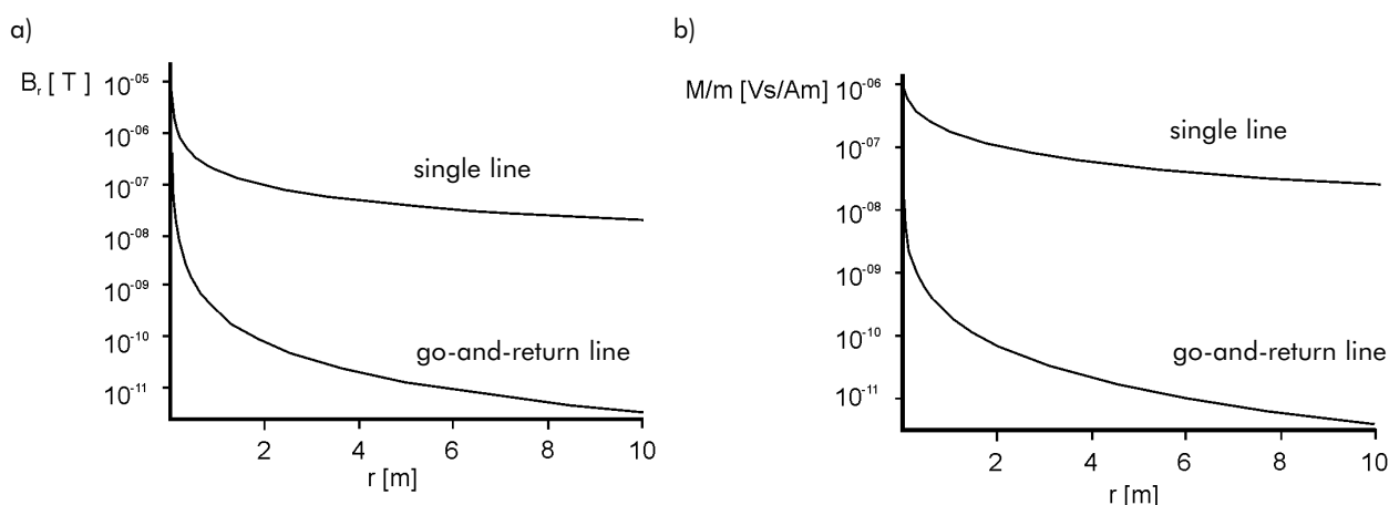
Figure 6 - a) the magnetic field of a single and a go-and-return line b) the coupling inductance per unit length of a loop to a single and a go-and-return.
