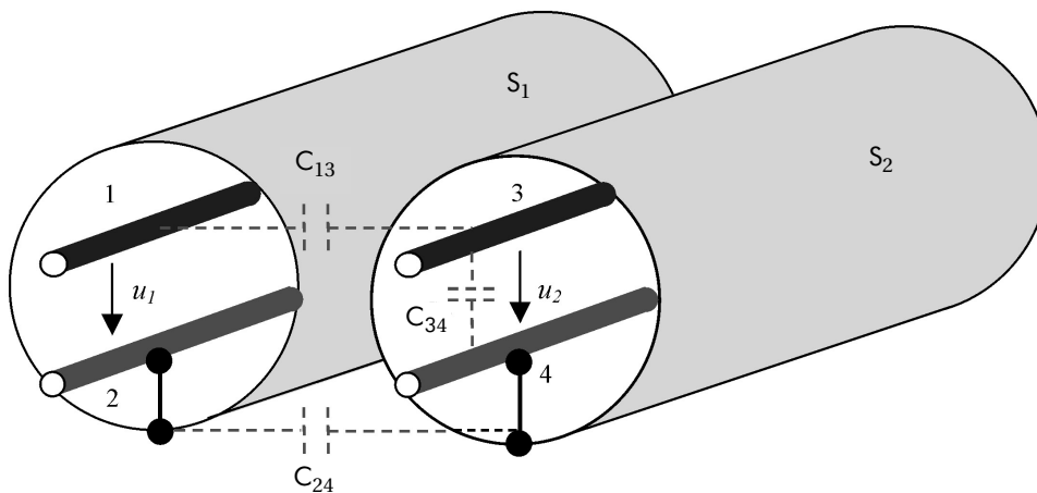
Figure 15 - Capacitive coupling of two shielded cables
