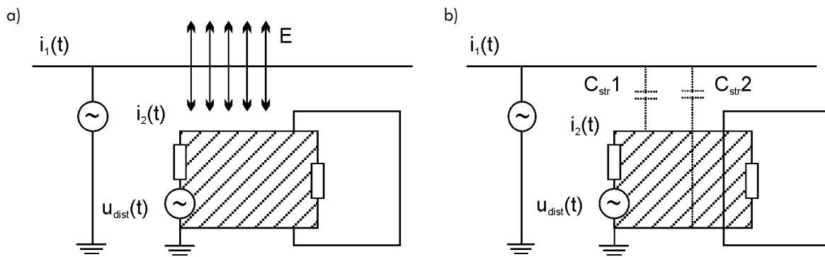
Figure 11 - Capacitive coupling a) field model, b) equivalent circuit
