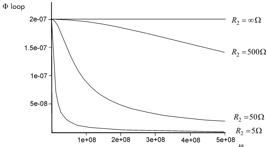
Figure 10 - Shielding effectiveness of a short circuit loop for various values of its resistance R_2
