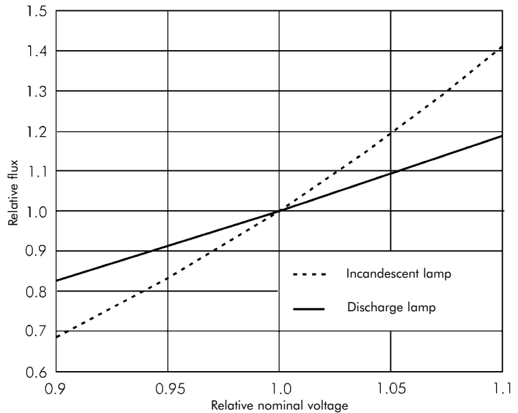
Figure 2 - Relative value of luminous flux F of an incandescent and discharge lamp as a function of the supply voltage according to formula (3)
