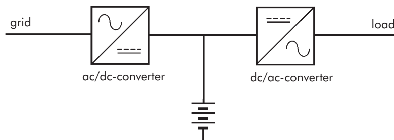
Figure 3 - Block diagram of a voltage frequency independent static UPS
