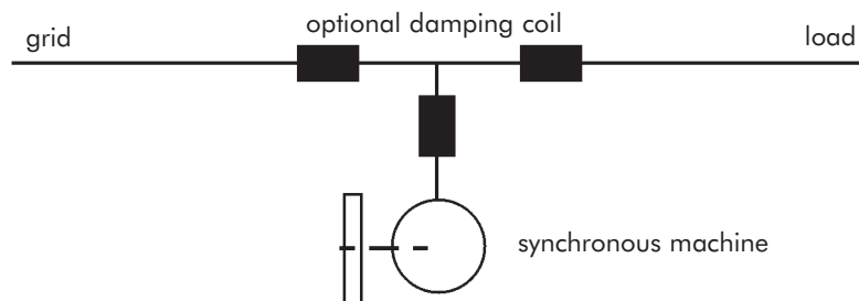
Figure 5 - Block diagram of shunt connected synchronous machine and flywheel
