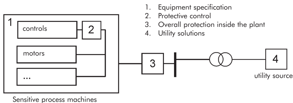
Figure 1- Possible mitigation methods [2]
