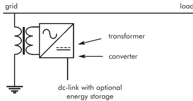
Figure 6 - Block diagram of a statcom
