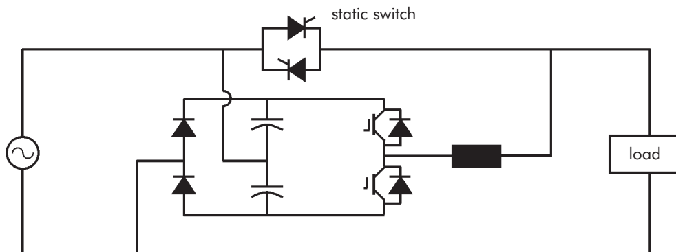
Figure 7 - Transformerless series injection
