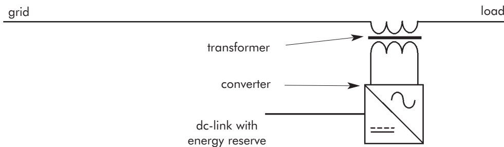
Figure 4 - Block diagram of a dynamic voltage restorer (DVR-2)
