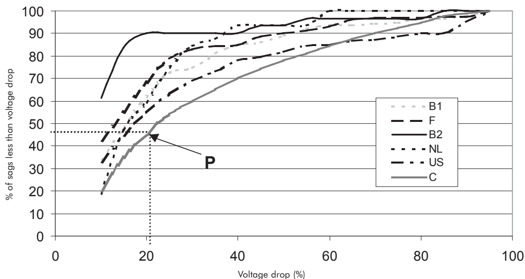
Figure 8 - Sag statistics from different countries, showing the percentage of sags less than a certain voltage drop in %
