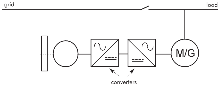
Figure 2 - Block diagram of a ride-through system using a flywheel
