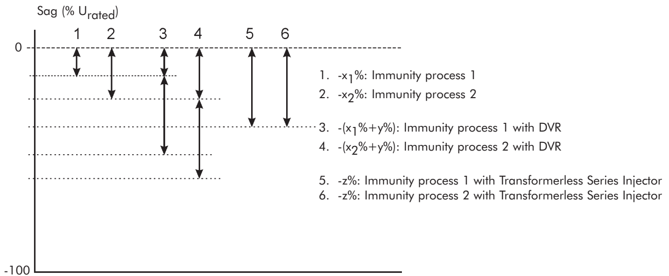
Figure 9 - Immunity of processes with different initial immunity with and without additional immunization equipment
