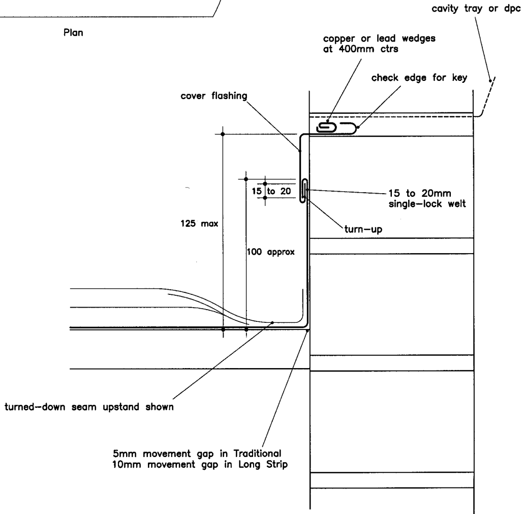
Fig 11a Vertical upstand 125mm max with horizontal cover flashing to brickwork TRADITIONAL ✓ LONG STRIP ✗
