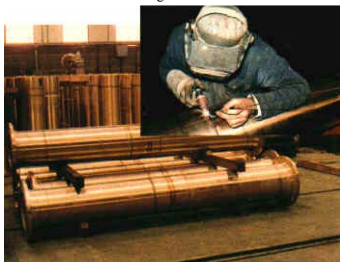
Figure 14 – Spuncast aluminium bronze pipes for offshore platform. Cast with a flange on one end, after proof machining and joint preparation, welded, stress relieved and non-destructively tested.
