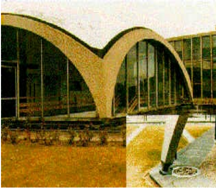
Figure 4 – Dome roof supported on aluminium bronze spherical joints
