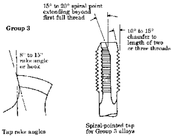
Tap rake angles
