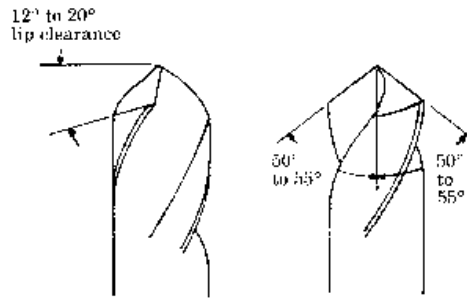
Drill point and clearance angles.
